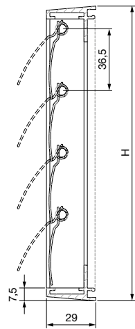
Renson® Technology extractor hood louvre 433/S
